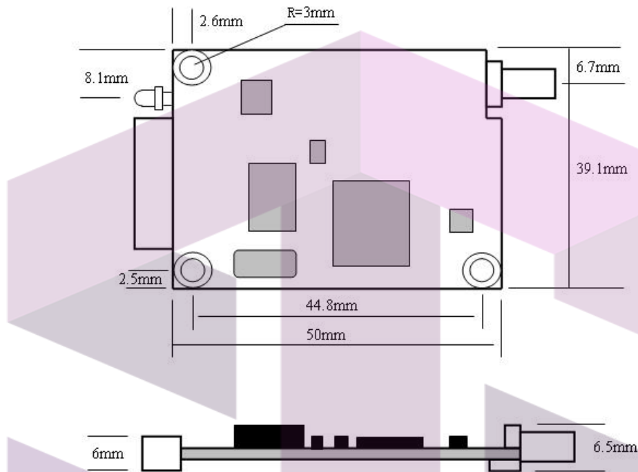
Figure 4: Mechanical Dimensions
